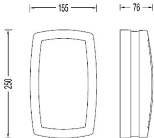
Dimensional Drawings
