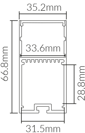
Dimensional Drawings
