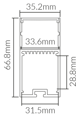
Dimensional Drawings
