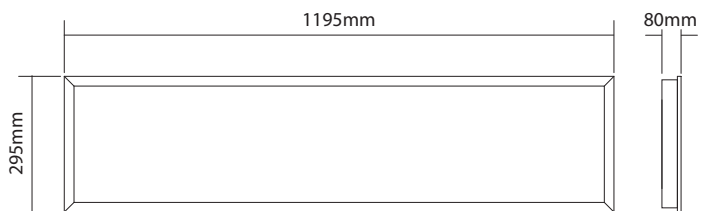
Dimensional Drawing
