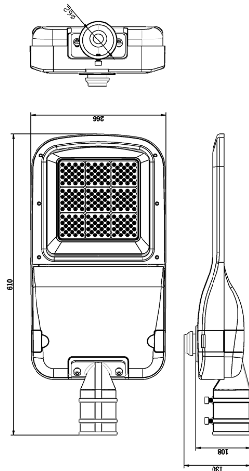
Dimensional Drawings
