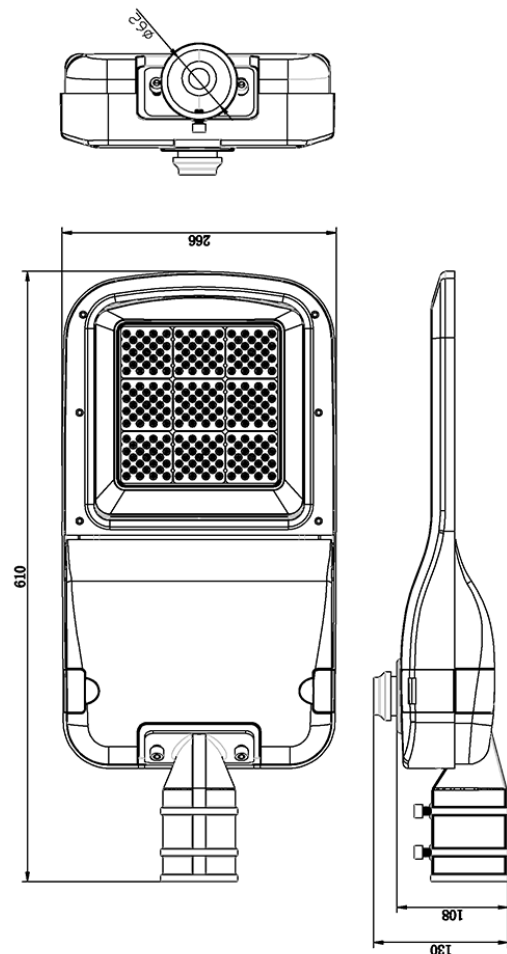
Dimensional Drawings
