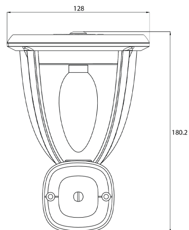
Dimensional Drawings
